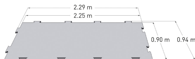
Dimensions sheet
